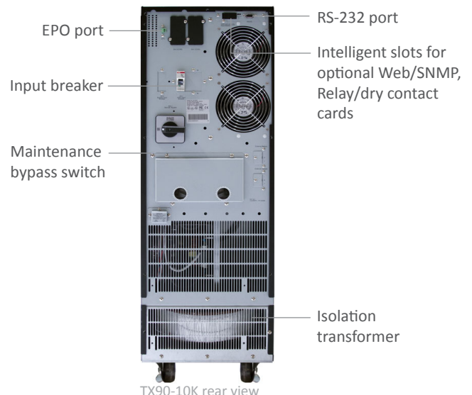
TX90-10K rear view
