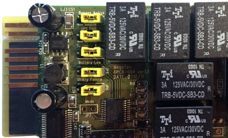
Jumper setting for Active Open
