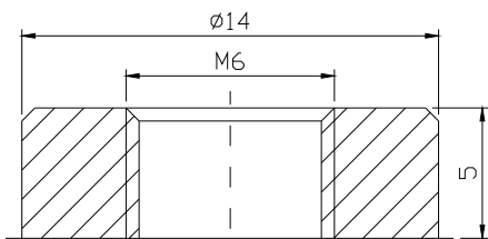
Terminal 6 mm Torque 6 NM / 53in/lbs
