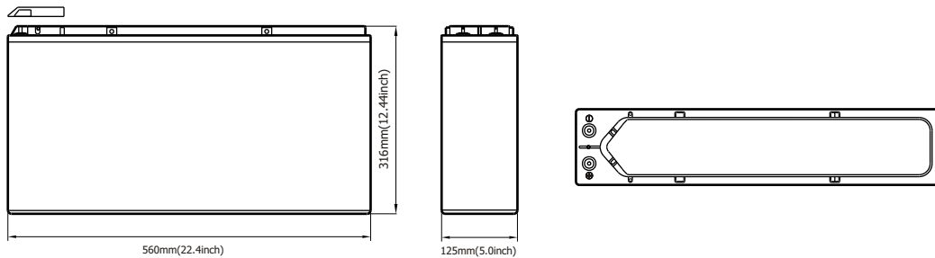
Terminal 8 mm Torque 8 NM / 71in/lbs
